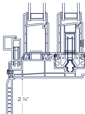
2 1/4" Contoured Z-Bar
