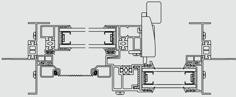
Horizontal Detail
