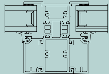
Integral Mullion detail to create multiple lite picture windows
