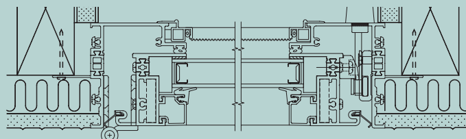
Casement Detail
