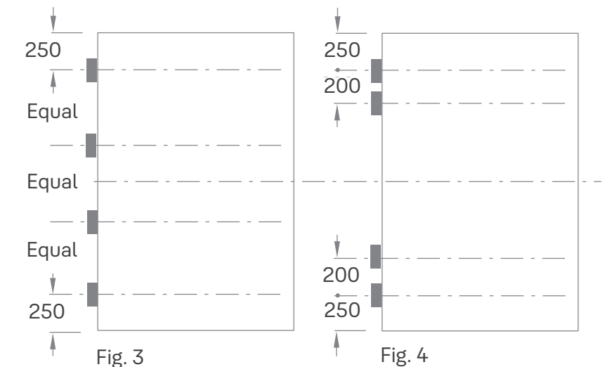
Doors over 2,100 height (4 hinges)
