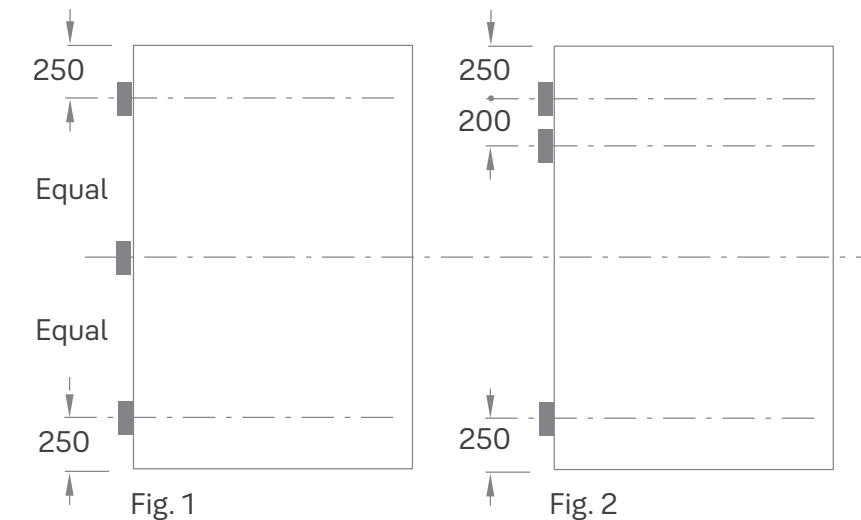
Doors up to 2,100 height (3 hinges)
