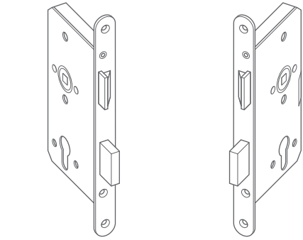
DIN left hand lock (the straight side of the latch points to the left)
