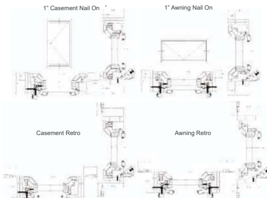
Casement and Awning - Frame Cross Sections
