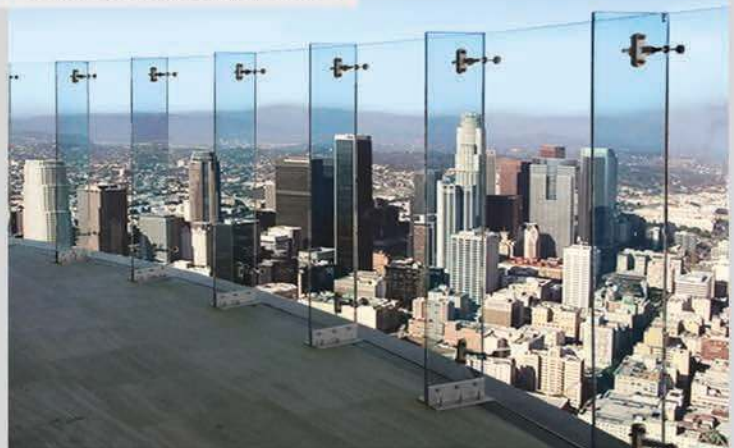
Structural Safe Laminated Glass with Custom Brackets & Spiders
