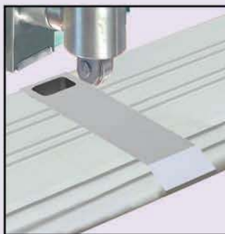
6b- T-HOLD STRIKE (PL 110 ONLY)
