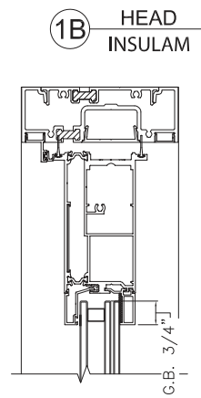
Insulating Laminated
